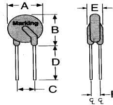
FBR 550-90 ~ FBR 900-90 Lead Size : 20AWG Φ 0.81 mm Diameter
