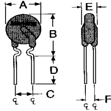
FBR 100-90 ~ FBR 350-90 Lead Size : 24AWG Φ 0.51 mm Diameter
